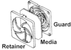
551147 Finger Guard
